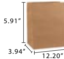
#8 SOS Non-Handle Kraft Paper Bag Item Code: 71008 SCC Code: 10628295001945 Pack Size: 500pcsx1pack=500
