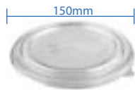
PET Dome Lid for 150mm Container Item Code: 56251DL SCC Code: 10628295003451 Pack Size: 45pcsx8pack=360
